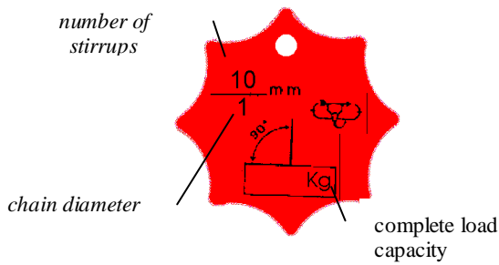
nominal diameter and load capacity for chains
